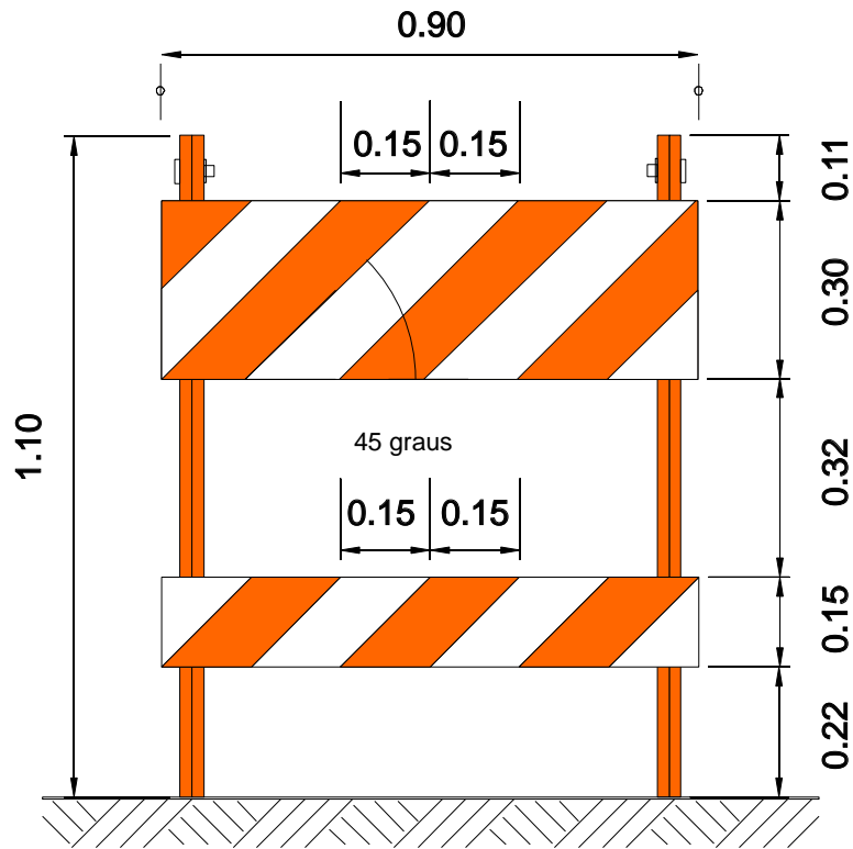
VISTA FRONTAL
